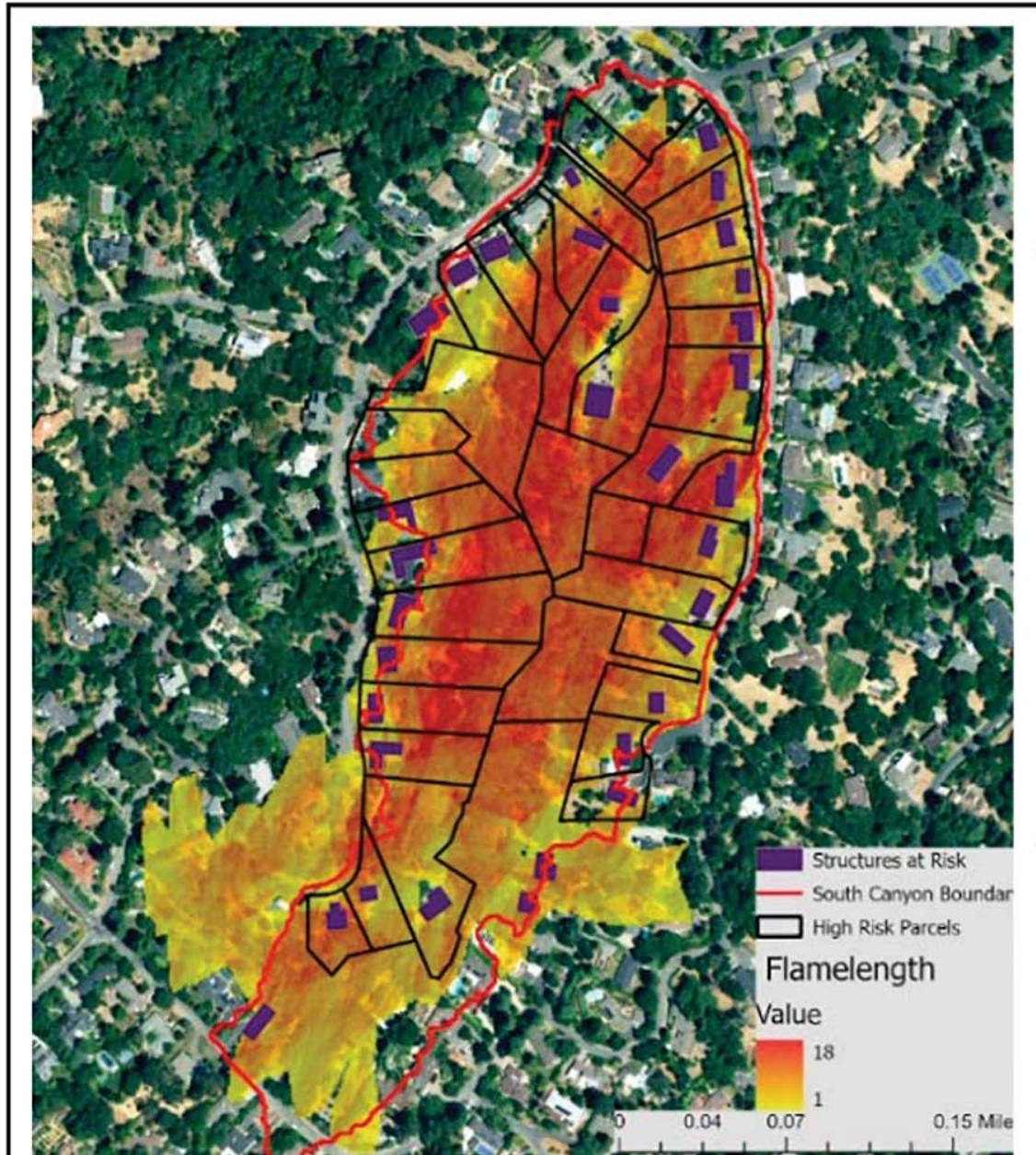
Figure 10: Prototype fireshed neighborhood simulated Flame Length (Raine, 2022)
